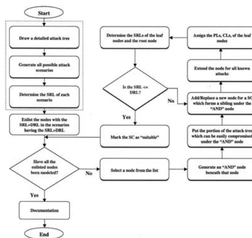
Figure 3. Evaluation method for security controls.
